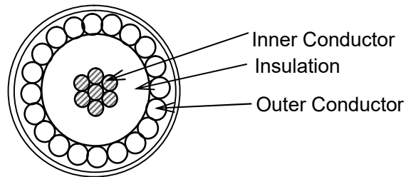
Fig.1 Cross section view of cable (32AWG Coaxial )
